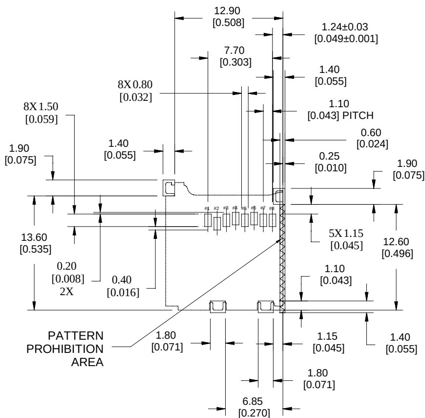
RECOMMENDED PCB PATTERN LAYOUT \pm 0.05 [0.002]
